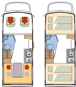
Ontario 600 H
