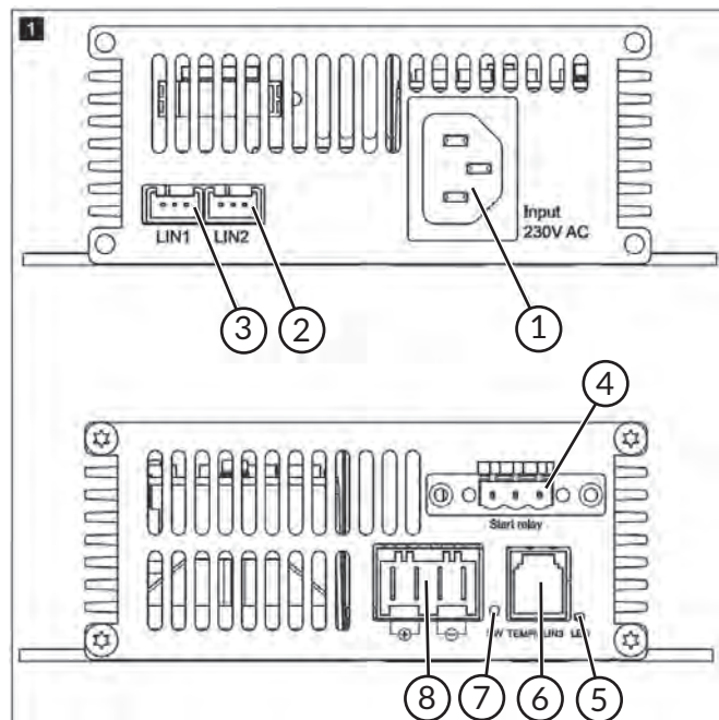
Raccordements chargeur
