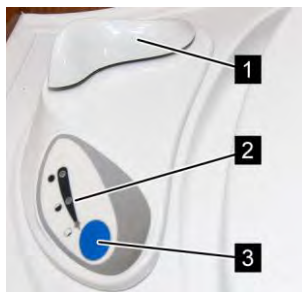
Control panel
