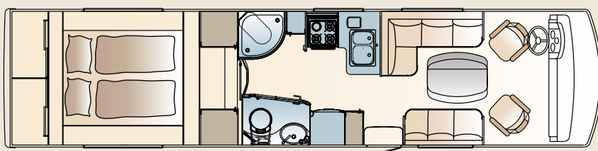
I 9800 QD-Car
