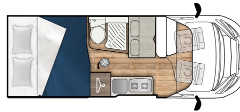
E-Van DUO XL Premium/Trend ↔ 6360 mm
