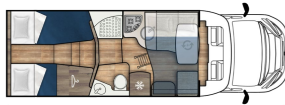
Baron 573 ← 7450 mm I 2350 mm
