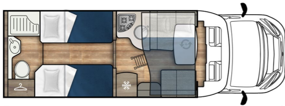
Baron 575 ← 7430 mm I 2350 mm
