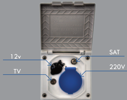
Multifunction external socket for TV, 12V, 220V and Satellite
